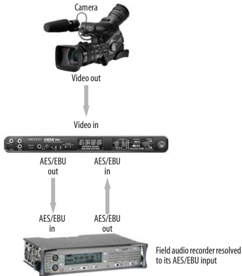
Figure 3-12: Capturing digital audio from a third device that is not the current video source. In this case, the third device must resolve to the HDX-SDI via its AES/EBU input.
