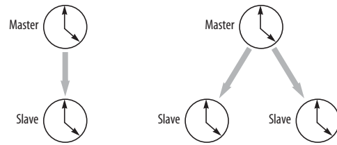
Figure 3-11: Without sample rate conversion, you need to choose a clock master to which all other devices slave. Each slaved device remains continuously resolved to the master, meaning that there will be no drift over time.
