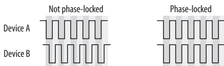
Figure 3-10: When transferring audio without sample rate conversion, two devices must have phased-locked audio clocks to prevent clicks, pops or other artifacts.
