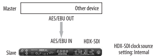
Figure 3-13: Rate-converting AES/EBU input.
