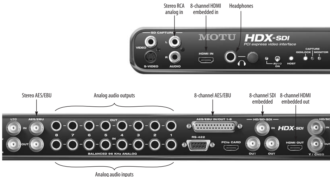
Figure 3-5: The HDX-SDI audio connectors.
