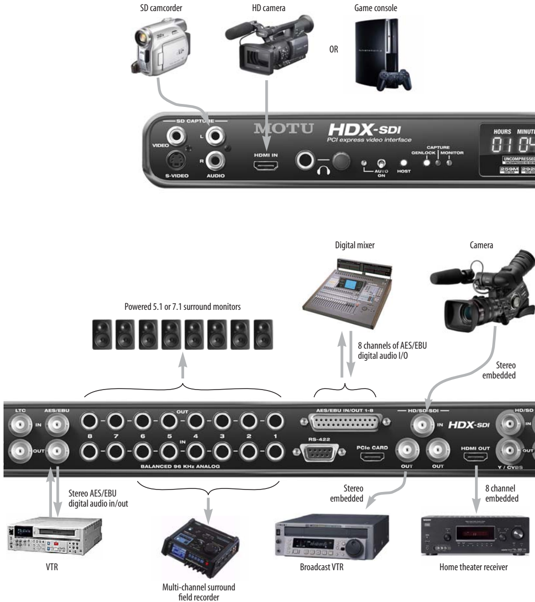
Figure 3-7: HDX-SDI audio connections.
